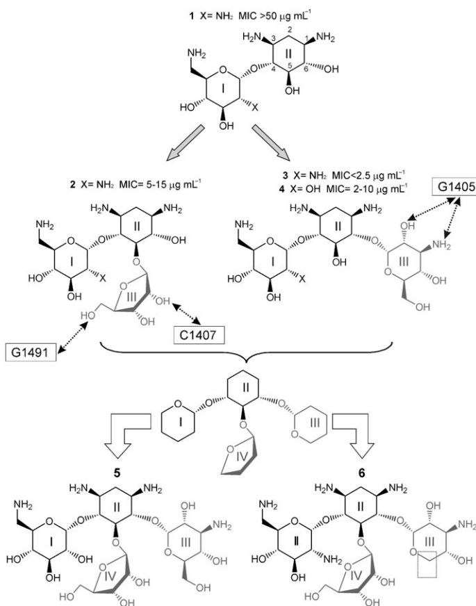
Scheme 1. The general strategy employed in the design of a new family of antibiotics. The pseudodisaccharide fragment common to most aminoglycosides is represented at the top. Addition of a sugar ring (grey) at the 5- or 6-position of the aminocyclitol unit gives rise to the 4,5-DOS (left) and 4,6-DOS (right) subfamilies, respectively. The functional relevance of the additional drug/RNA contacts established through ring III (indicated in each case) is reflected in the antibiotic activities (typical ranges for the MIC values are also presented for comparison). We propose the synthesis and evaluation of the highly crowded new derivatives 5 and 6 , which incorporate the trisubstituted 2-DOS scaffold. The ribose unit, numbered as III in ribostamycin ( 2 ), has been renumbered as IV in the non-natural pseudotetracosaccharides.
