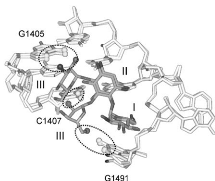
Figure 1. As shown by X-ray studies, the disaccharides I/II, present in both kanamycin-A and ribostamycin, occupy nearly identical positions within the RNA binding pocket. A superposition of kanamycin-A and ribostamycin I/II fragments in the complex is shown. Aminoglycoside/RNA contacts established through sugar unit III in both cases are highlighted.
