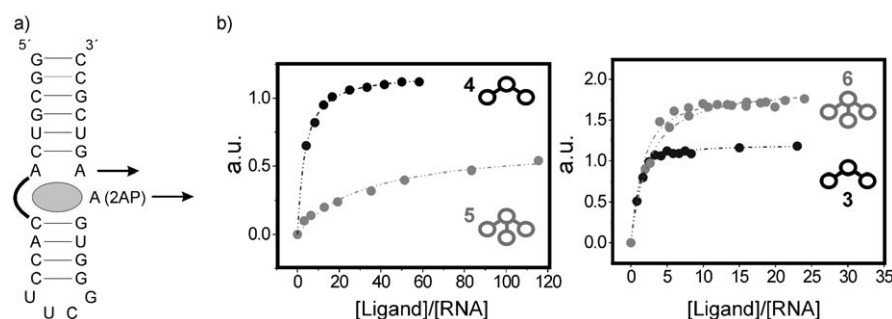
Figure 2. a) Schematic representation of the modified RNA fragment employed in our binding studies and the structural change induced by the ligand binding. b) Some representative binding curves obtained for natural aminoglycosides 3 and 4 (black) and the related pseudotetrasaccharides 5 and 6 (grey).
