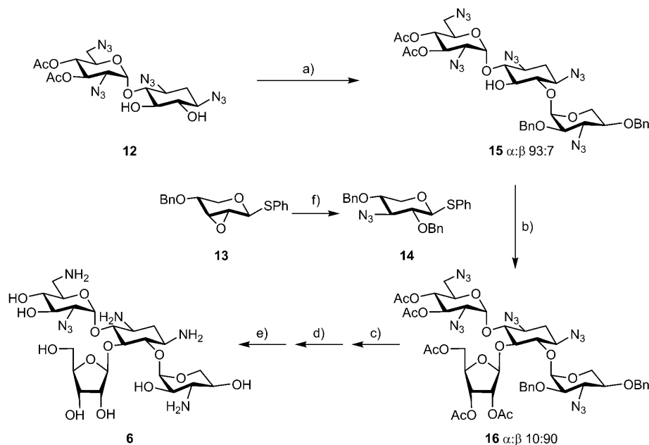
Scheme 3. Methodology employed for the synthesis of 6 . a) Glycosyl donor 14 , \text{TiOH} , NIS, \text{CH}_2\text{Cl}_2/\text{Et}_2\text{O} , -40^{\circ}\text{C} , yield: 89%; b) \text{BF}_3\cdot\text{Et}_2\text{O} , \text{CH}_2\text{Cl}_2 , -25 to -20^{\circ}\text{C} , glycosyl donor 10 , yield 41%; c) \text{MeONa} , \text{MeOH}/\text{THF} , 2 h; d) \text{Me}_3\text{P} , \text{THF} , \text{NaOH} , 24 h, 55^{\circ}\text{C} ; e) \text{H}_2 , \text{Pd/C} , \text{H}_2\text{O}/\text{AcOH} ; yield 35% (global yield for steps c–e); f) 1. \text{NaN}_3/\text{DMF} ; 2. benzylolation; yield 42%.
