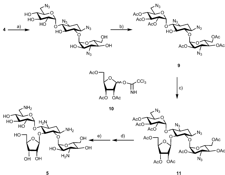
Scheme 2. Methodology employed for the synthesis of 5 . a) 1. Amberlite 400 ( \text{OH}^- ), \text{H}_2\text{O} , RT, 3 h; 2. \text{TfN}_3 , \text{CuSO}_4 , toluene/MeOH/py, RT, 16 h; b) \text{Ac}_2\text{O} , DMAP, py, RT, over night, yield: 80% (global yield for steps a and b); c) \text{BF}_3\cdot\text{Et}_2\text{O} , \text{CH}_2\text{Cl}_2 , -25 to -20^\circ\text{C} , glycosyl donor 10 , yield: 30%; d) \text{MeONa} , MeOH/THF, 2 h; e) \text{Me}_3\text{P} , THF, NaOH, 24 h, 55^\circ\text{C} , yield: 37% (global yield for steps d and e).
