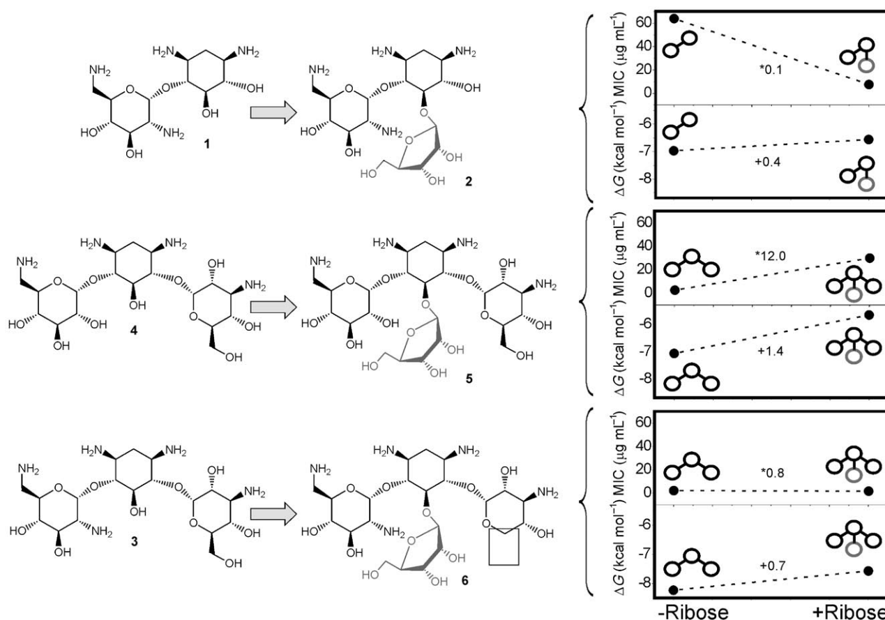
Figure 3. The aminoglycoside/RNA complex stabilities ( \Delta G ) and biological activities (MIC values) measured for several natural and non-natural aminoglycosides, with (right) and without (left) a neutral ribose unit (grey) at the 5-position of the 2-DOS ring, are represented.
